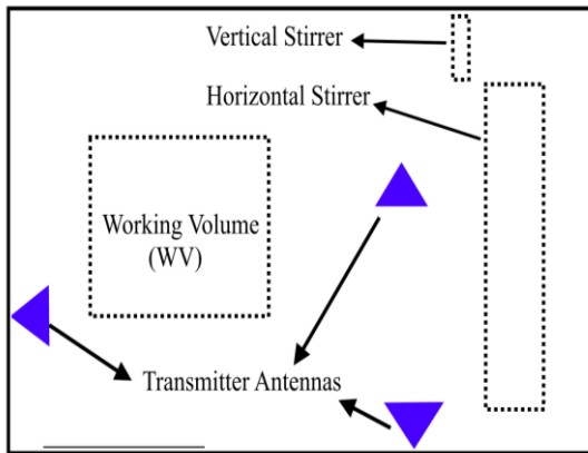
Fig 1 Main components of a RC
