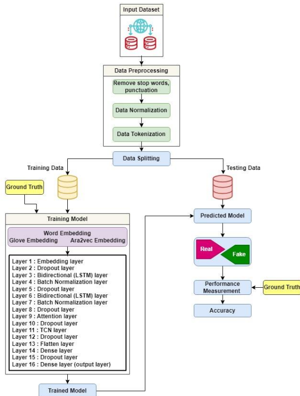
Fig.3: Proposed Model
