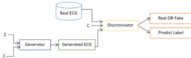
Fig. 1 Conditional GAN
