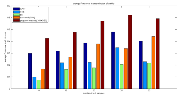
Fig. 9. Average F-measure of the Proposed Method
